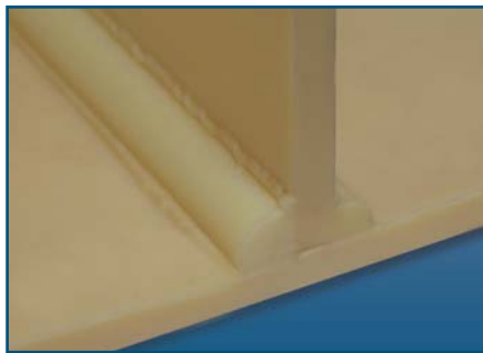
Electrode Weld on standard flat belt cleat
