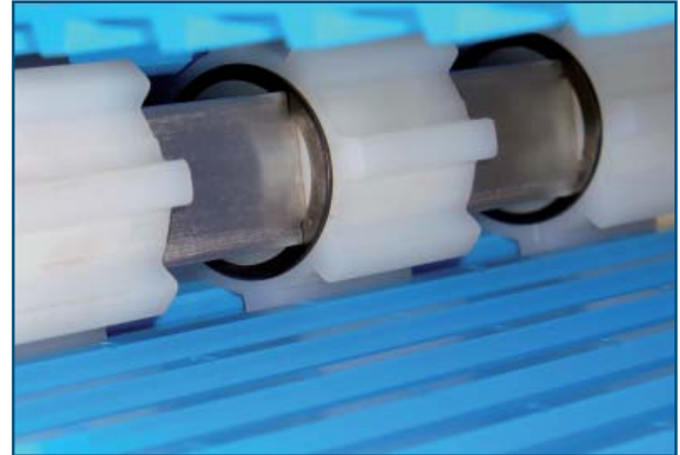
DualDrive SP pulleys: 50 mm diameter (8 teeth)
