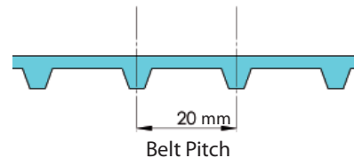
DualDrive SP pulleys: 50 mm diameter (8 teeth)
